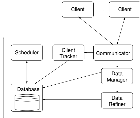
Fig. 3. Server architecture
