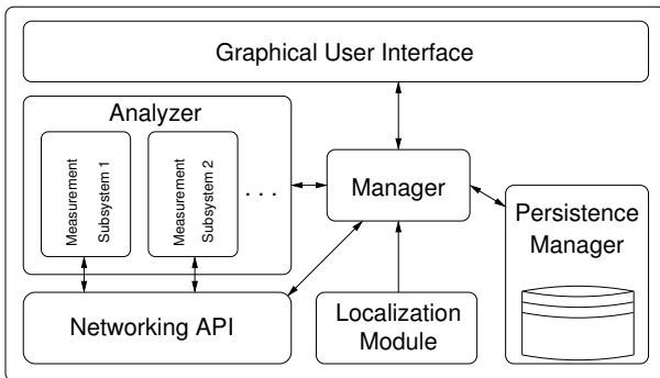
Fig. 2. Client architecture
